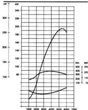
Full-Power Performance Turbo
