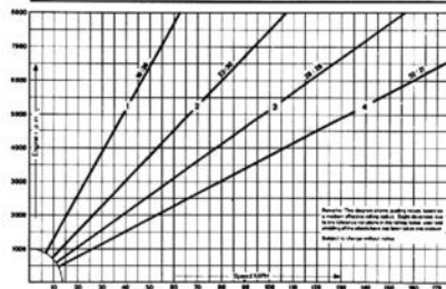
Transmission Diagram Turbo 4-speed-transmission
