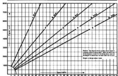
Transmission Diagram 911 SC 5-speed-transmission
