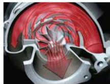
Guide vanes closed
