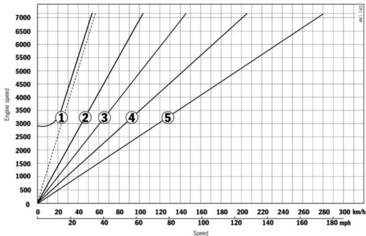
Boxster: Transmission diagram Tiptronic
