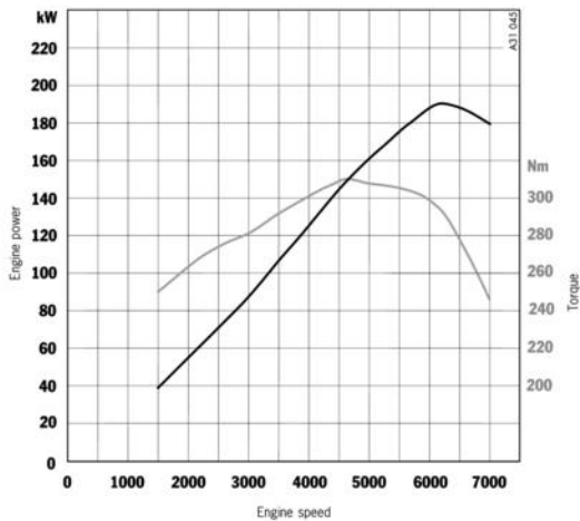
Boxster S: Engine diagram at full power
