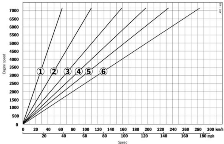
Boxster S: Transmission diagram Manual transmission
