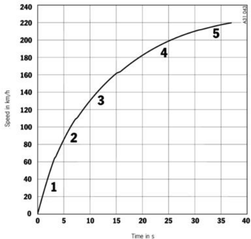
Boxster: Acceleration diagram Manual transmission
