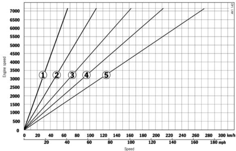
Boxster: Transmission diagram Manual transmission
