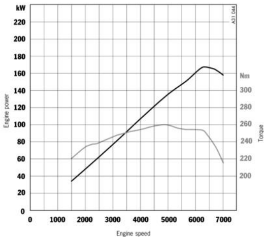
Boxster: Engine diagram at full power
