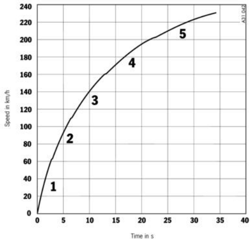
Boxster S: Acceleration diagram Manual transmission
