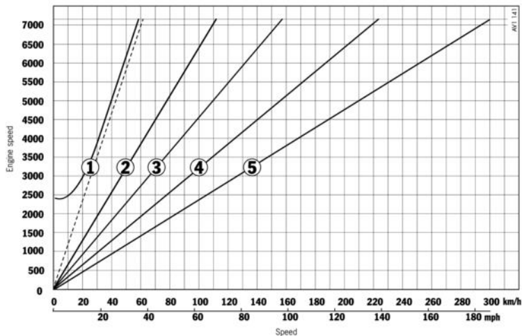
Boxster S: Transmission diagram Tiptronic
