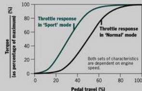
Comparison of electronic and throttle maps for 'Normal' and 'Sport' mode
