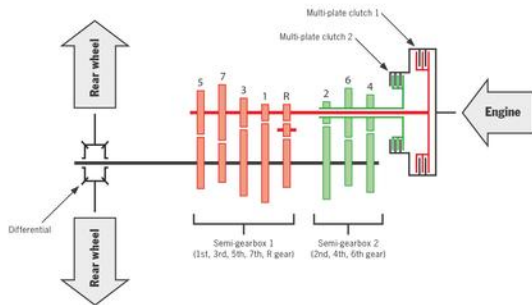
PDK function diagram
